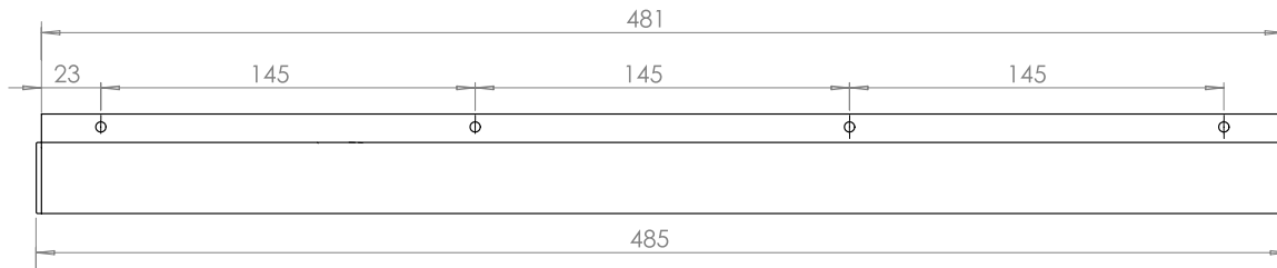
FIGURE 18. MGSW4800 Dimensions
