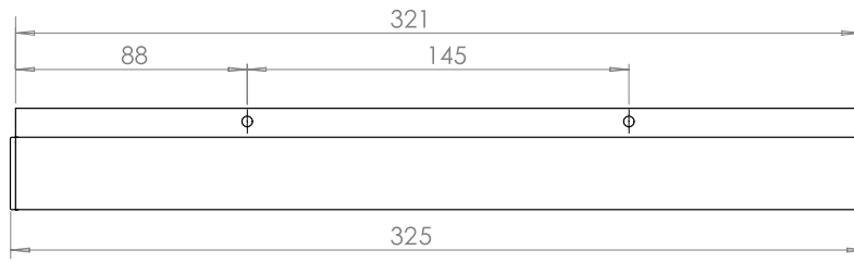
FIGURE 17. MGSW3200 Dimensions
