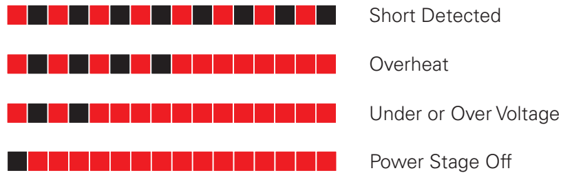
FIGURE 10. Exception or Fault Flashing Patterns
