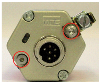
Fig. 2: Fasten screws with 1,3 Nm
