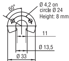
U-Magnet M OD33 Part No. 251 416-2
